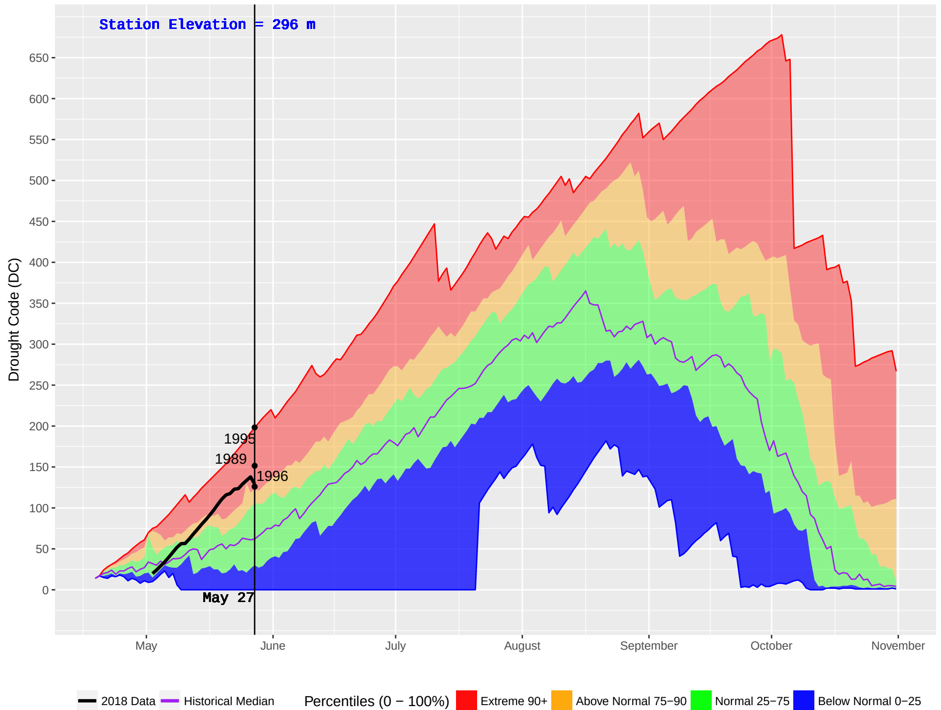
VAN DYKE (430) : Historical (1983–2016) and Current (2018) Noon Drought Code (DC)
