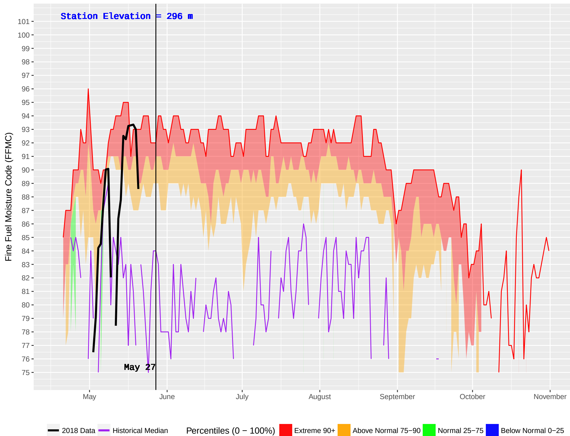
VAN DYKE (430) : Historical (1983–2016) and Current (2018) Noon Fine Fuel Moisture Code (FFMC)
