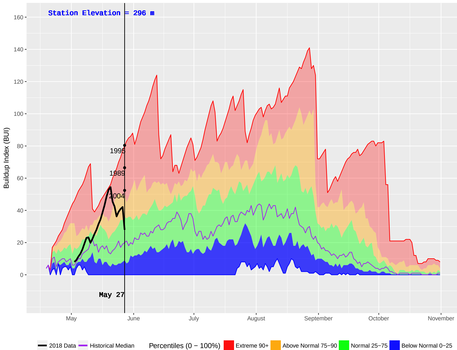
VAN DYKE (430) : Historical (1983–2016) and Current (2018) Noon Buildup Index (BUI)
