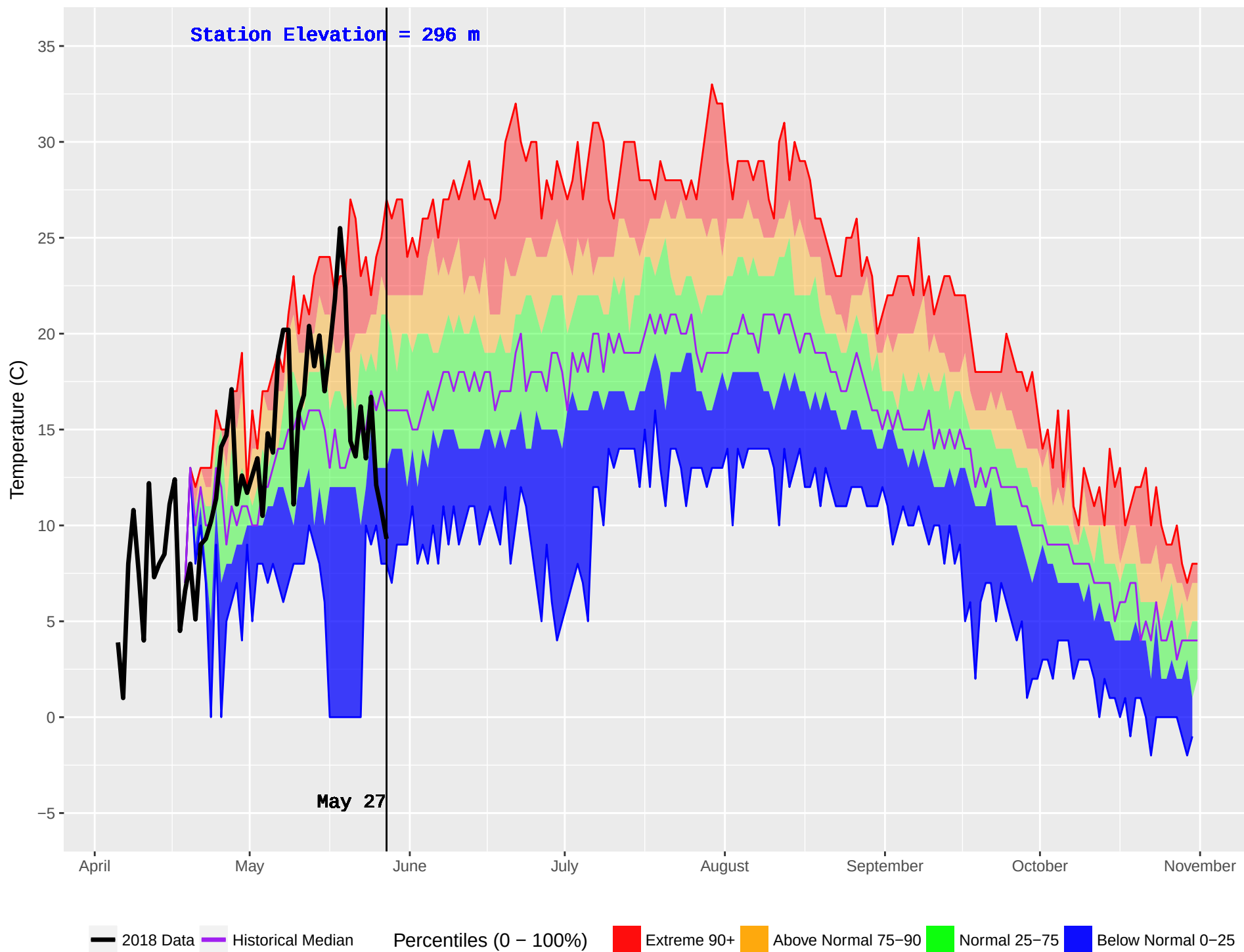
VAN DYKE (430) : Historical (1983–2016) and Current (2018) Noon Temperature
